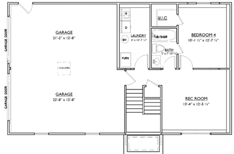
Lower Level (566 +/- SF Finished & 578 +/- SF Garage)
